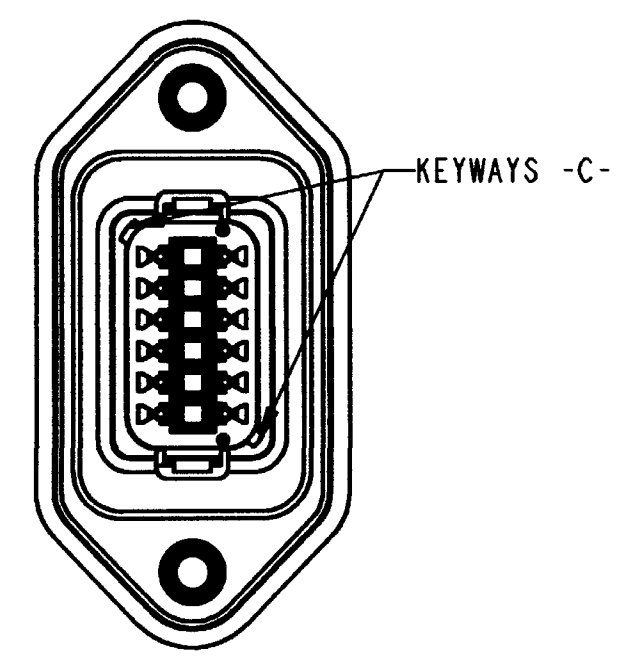
DT04-12PC-LE01 KEY ARR. -C- COLOR : GREEN (SHELL AND WELD CAP)
