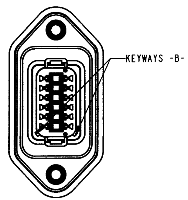
DT04-12PB-LE01 KEY ARR. -B- COLOR : BLACK (SHELL AND WELD CAP)
