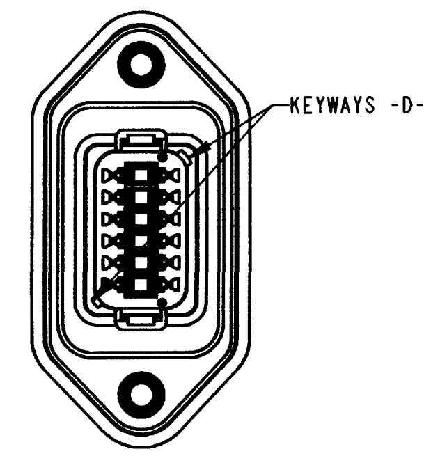
DT04-12PD-LE01 KEY ARR. -D- COLOR : BROWN (SHELL AND WELD CAP)
